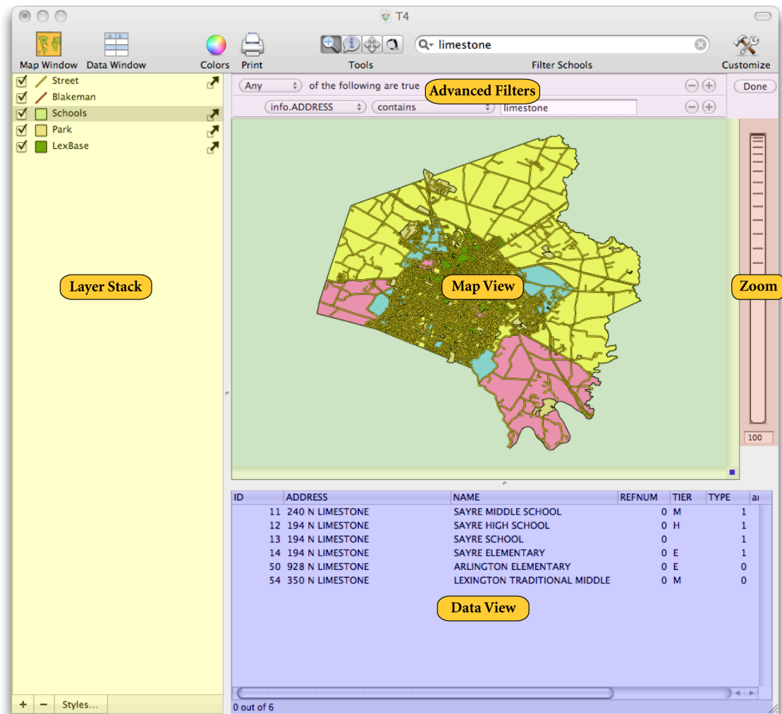
Figure 2.2. Main Cartographica window
